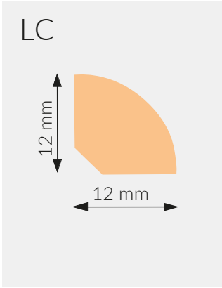
QUARTER ROUND PROFILE
